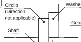
B Detail of installation of circlip
